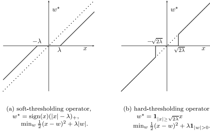
Fig. 1.6. Soft- and hard-thresholding operators.
