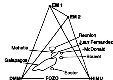
Fig. 1. Mantle tetrahedron from our report showing locations of additional high He 3 / 4 islands not shown in figure 1 of the comment by Farley and Craig. References for heavy isotope data may be found in (3); He data are from standard sources, Farley and Craig, and (1).
