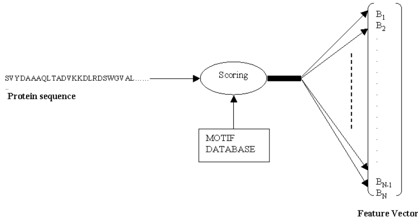
Figure 2: The procedure to generate feature vectors for proteins. B_i in the feature vector is the sum or maximum of the scores (depending on the approach) for the i th block in the motif database found in the protein.
