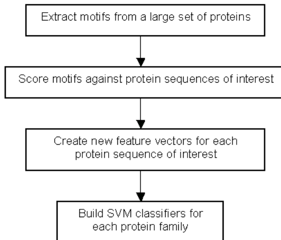
Figure 1: Overall Algorithm
