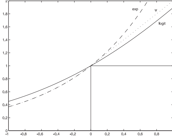
FIG. 1. Bounding the step function with different cost functions \phi = \text{exp}, \psi, \text{logit} .
