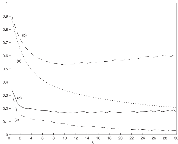
FIG. 3. Threenorm, cost \phi = \psi , n = 500 , m = 1000 ; plots of (a) A_n^\lambda(\hat{f}_n^\lambda) , (b) A^\lambda(\hat{f}_n^\lambda) , (c) training error and (d) test error.
