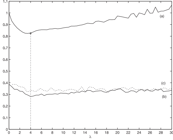
FIG. 5. Threernorm , cost \phi = \psi , \eta = 0.1 , n = 100 , m = 500 ; plot of (a) A^\lambda(\hat{f}_n^\lambda) with MARGINBOOST.L 1 for various \lambda 's, (b) test error with MARGINBOOST.L 1 for various \lambda 's and (c) test error with one run of MARGINBOOST (unnormalized weights) where the test error is plotted as a function of the sum of the weights of the combined classifier denoted by \lambda_T .
