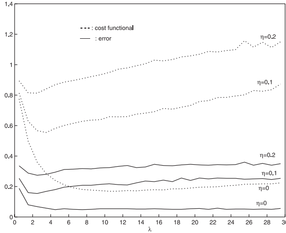
FIG. 4. Twonorm , cost \phi = \psi , n = 100 , m = 500 ; plots of A^\lambda(\hat{f}_n^\lambda) (dotted lines) and of the test error (solid lines) for levels of noise \eta = 0, 0.1, 0.2 .
