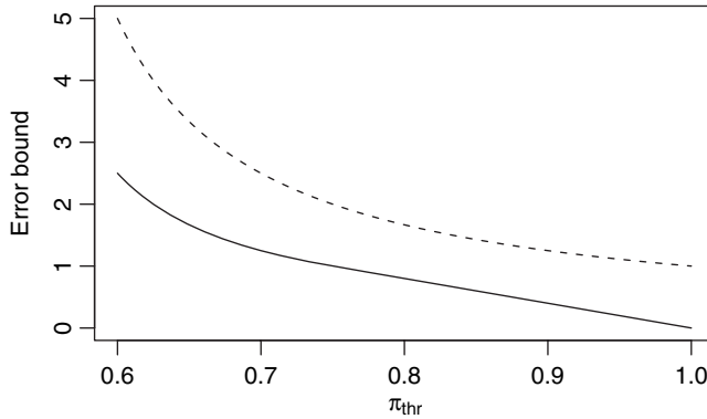
Fig. 14. Factor multiplying q_{\Lambda}^2/\rho against \pi_{thr} for each of the bounds: the bound of theorem 1 (-----) and the new bound with M = \infty (—)
