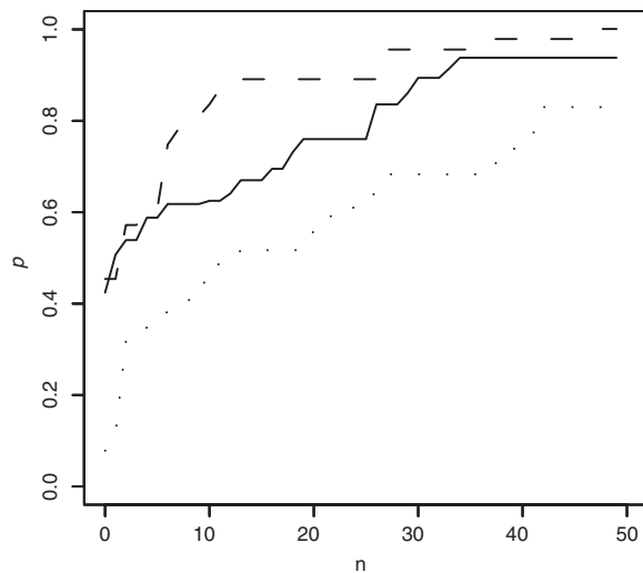
Fig. 5. Comparing three scoring functions for the regulatory T-cell data set. The x -axis has gene ranks, the y -axis has adjusted p -values. T\Sigma (dotted curve) yields better p -values than \Sigma T (solid curve) and \Sigma T rescaled (dashed curve). Same qualitative behavior occurs for the other two data sets.
