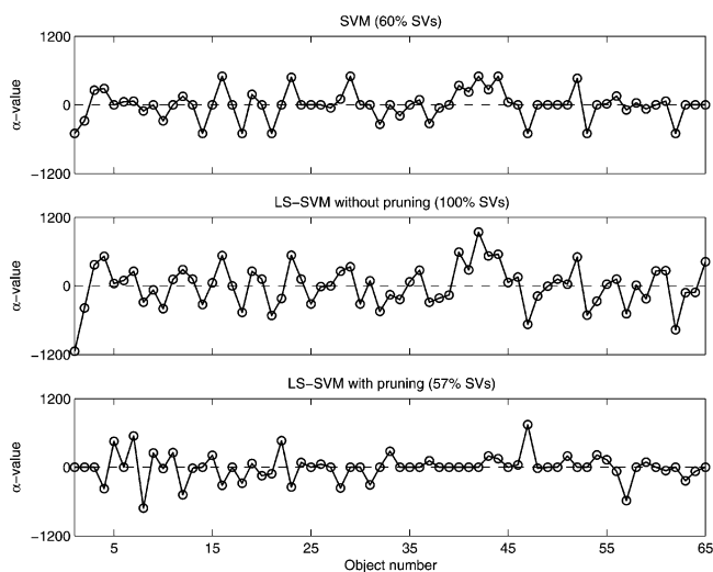
Figure 4. Values of the Lagrange multipliers from ethanol prediction models. The upper row shows the results for the SVM, while the middle and bottom rows show the Lagrange multipliers for LS-SVM and the pruned LS-SVM, respectively. Similar results are obtained for the prediction of water and 2-propanol.
