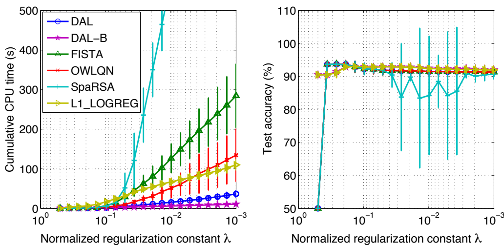
Figure 7: Dorothea data set ( m = 767, n = 100,000 ). DAL is efficient in this case ( m \ll n ).
