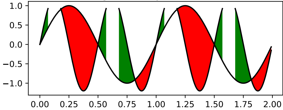
Now regions with y_2 > 1 are masked
