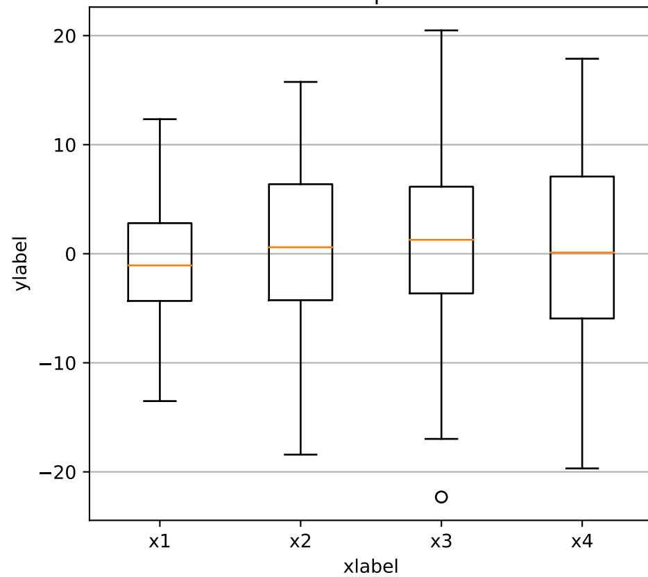
box plot
