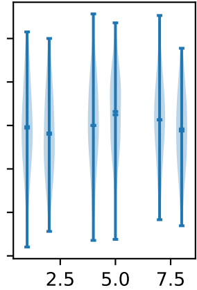
Custom violinplot 3
