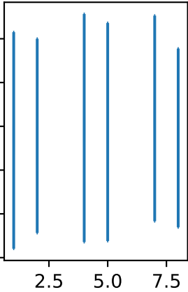
Custom violinplot 1
