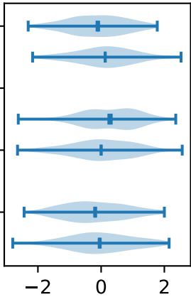
Custom violinplot 4
