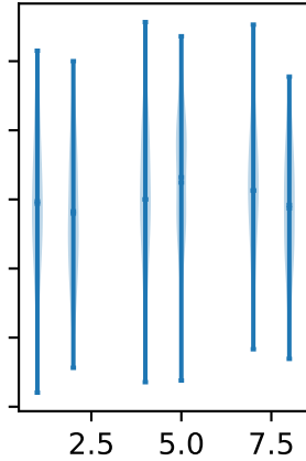
Custom violinplot 2
